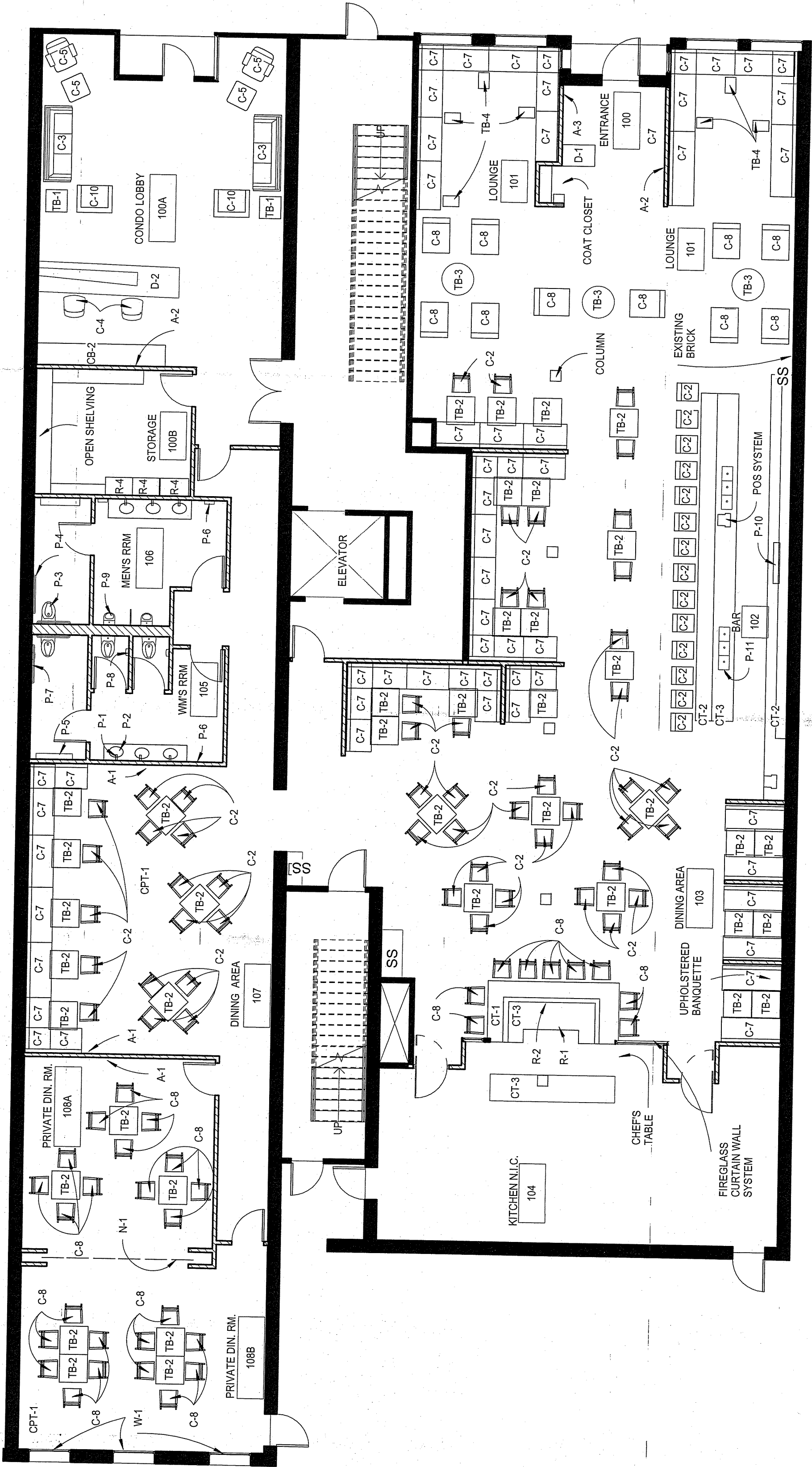
145 KENT 1ST FLOOR FIXTURES, FURNISHINGS & EQUIPMENT PLAN 1/8" = 1'-0"
