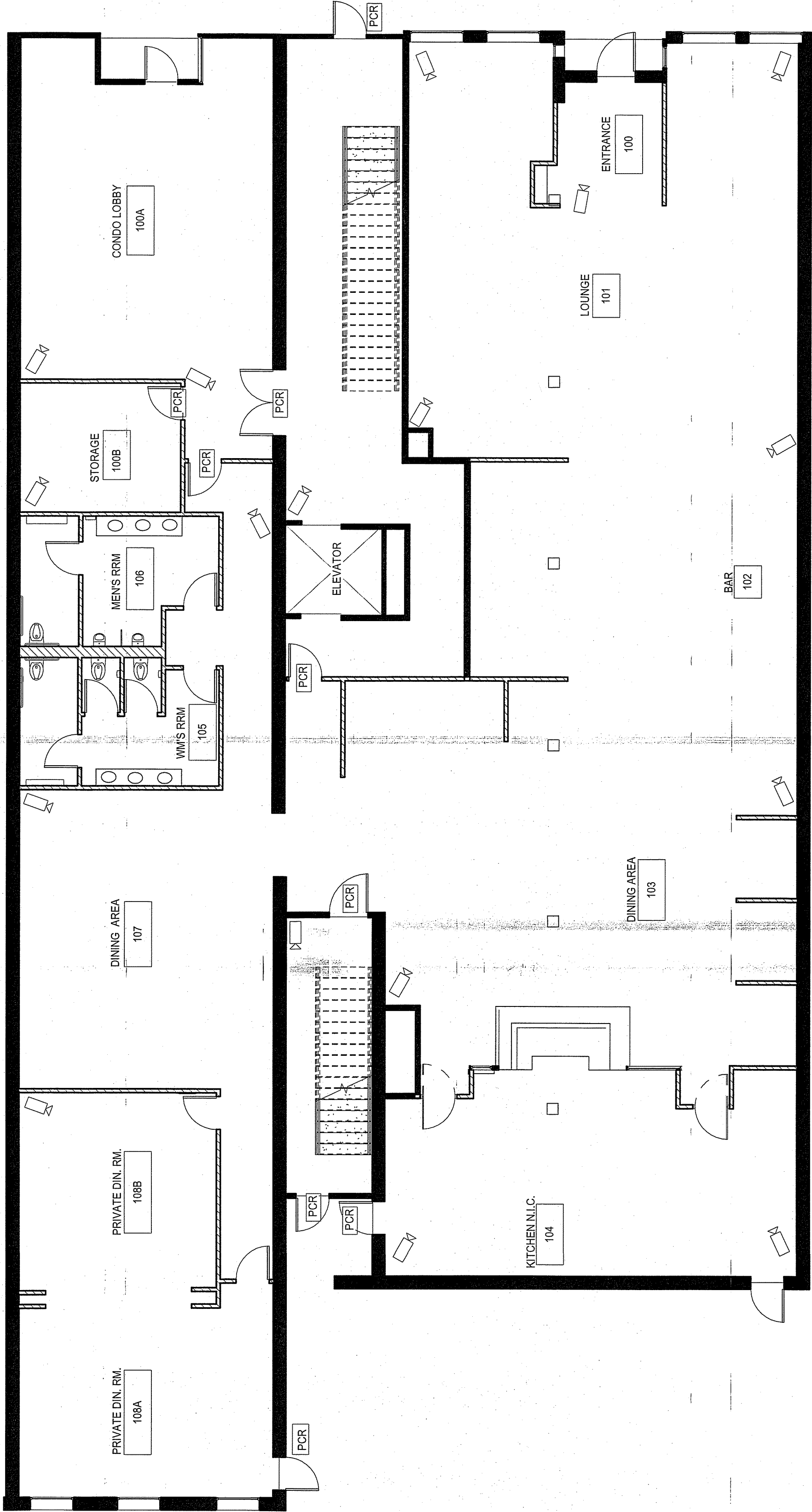
1 145 KENT 1ST FLOOR SECURITY PLAN 1/8" = 1'-0"
