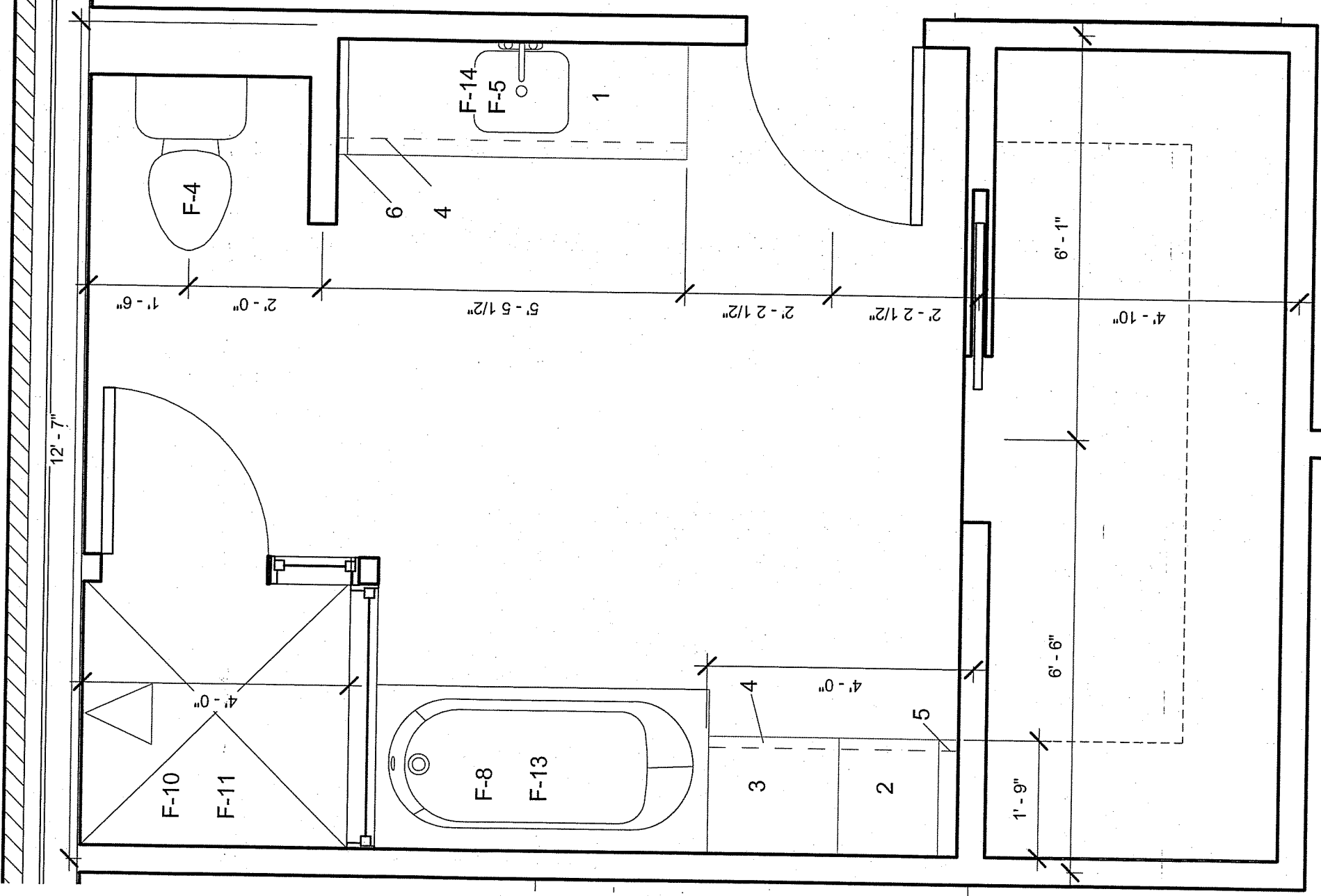
2 GIRLS BATHROOM LARGE SCALE PLAN 1/2" = 1'-0"
