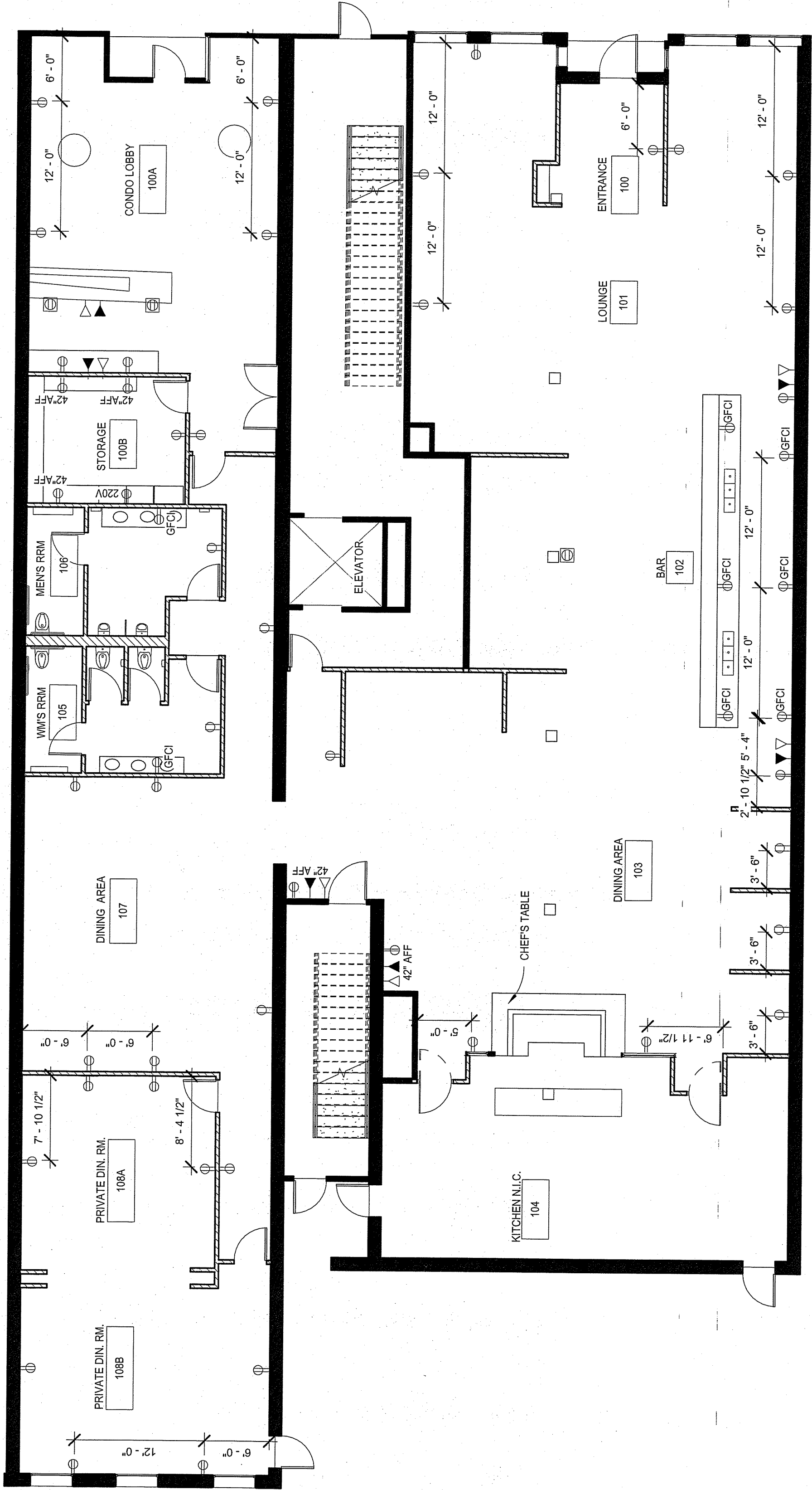
145 KENT 1ST FLOOR POWER & COMMUNICATION PLAN 1/8" = 1'-0"
