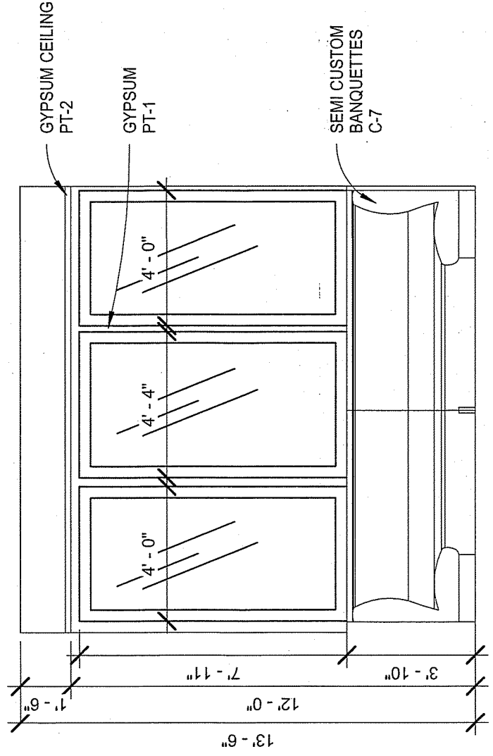
3 LOUNGE 1/4" = 1'-0"
