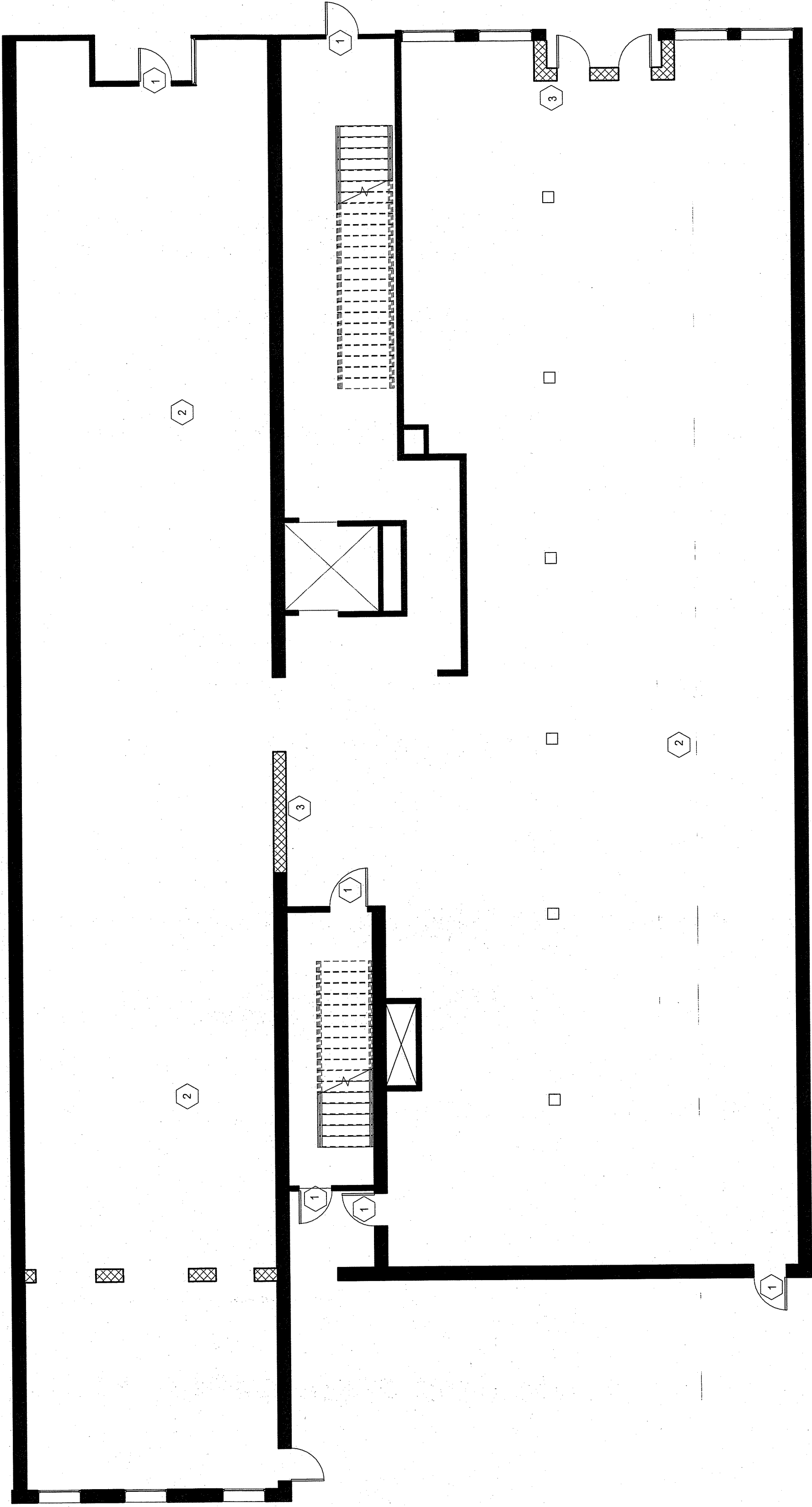
1 145 KENT 1st FLOOR DEMOLITION PLAN 1/8" = 1'-0"
