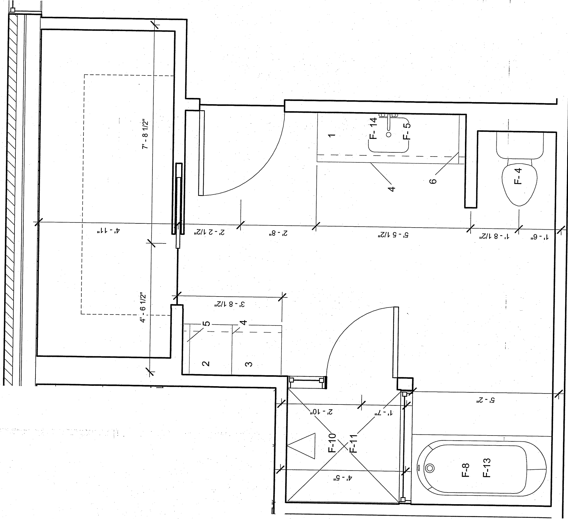
1 BOYS BATHROOM LARGE SCALE PLAN 1/2" = 1'-0"
